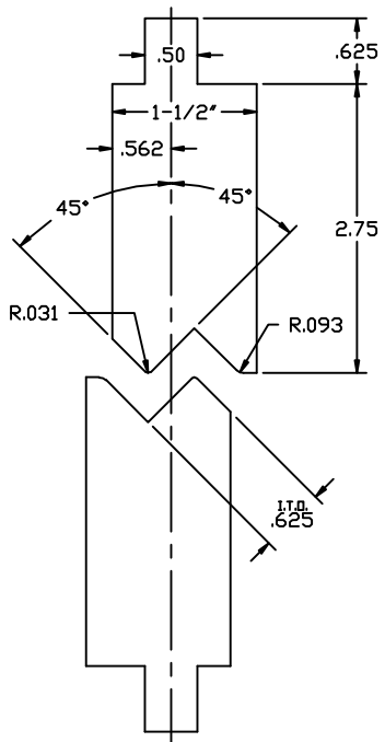
OS-5/8" 16 GAUGE
