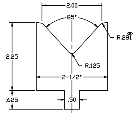
F-2" 1/4" CAPACITY
