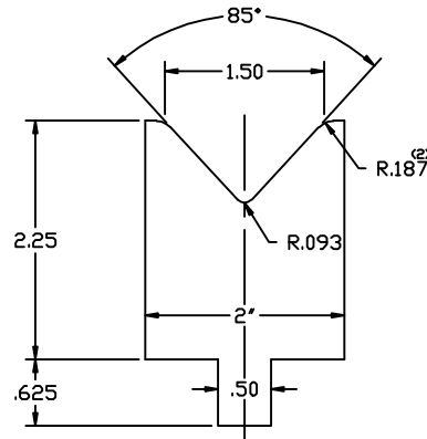
F-1 1/2" 3/16" CAPACITY
