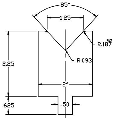
F-1 1/4" 9 GAUGE
